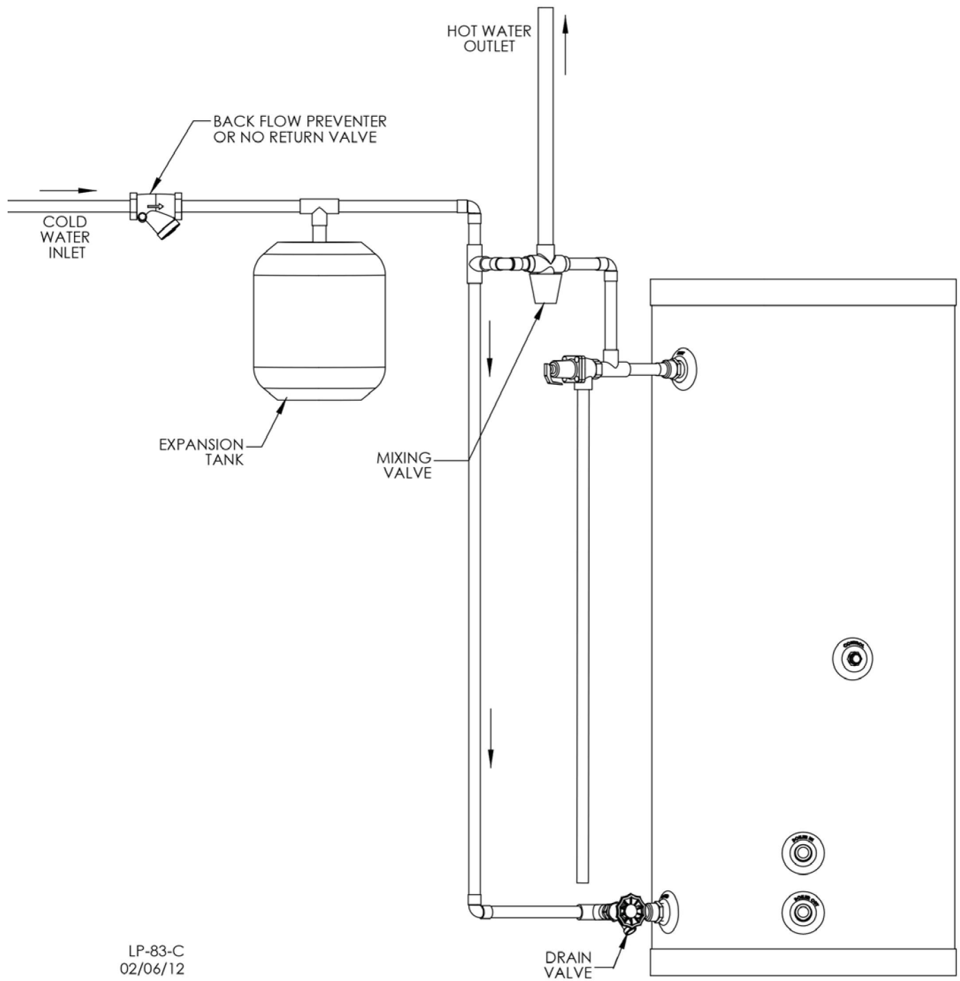
Hot Water Heater Piping Diagram
